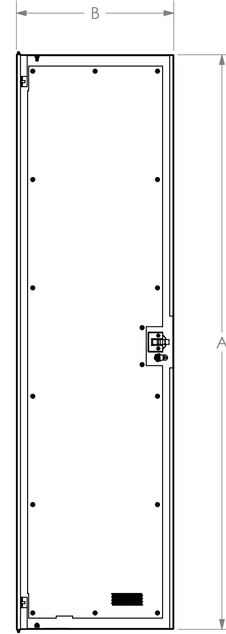
PERFERATED DOOR
