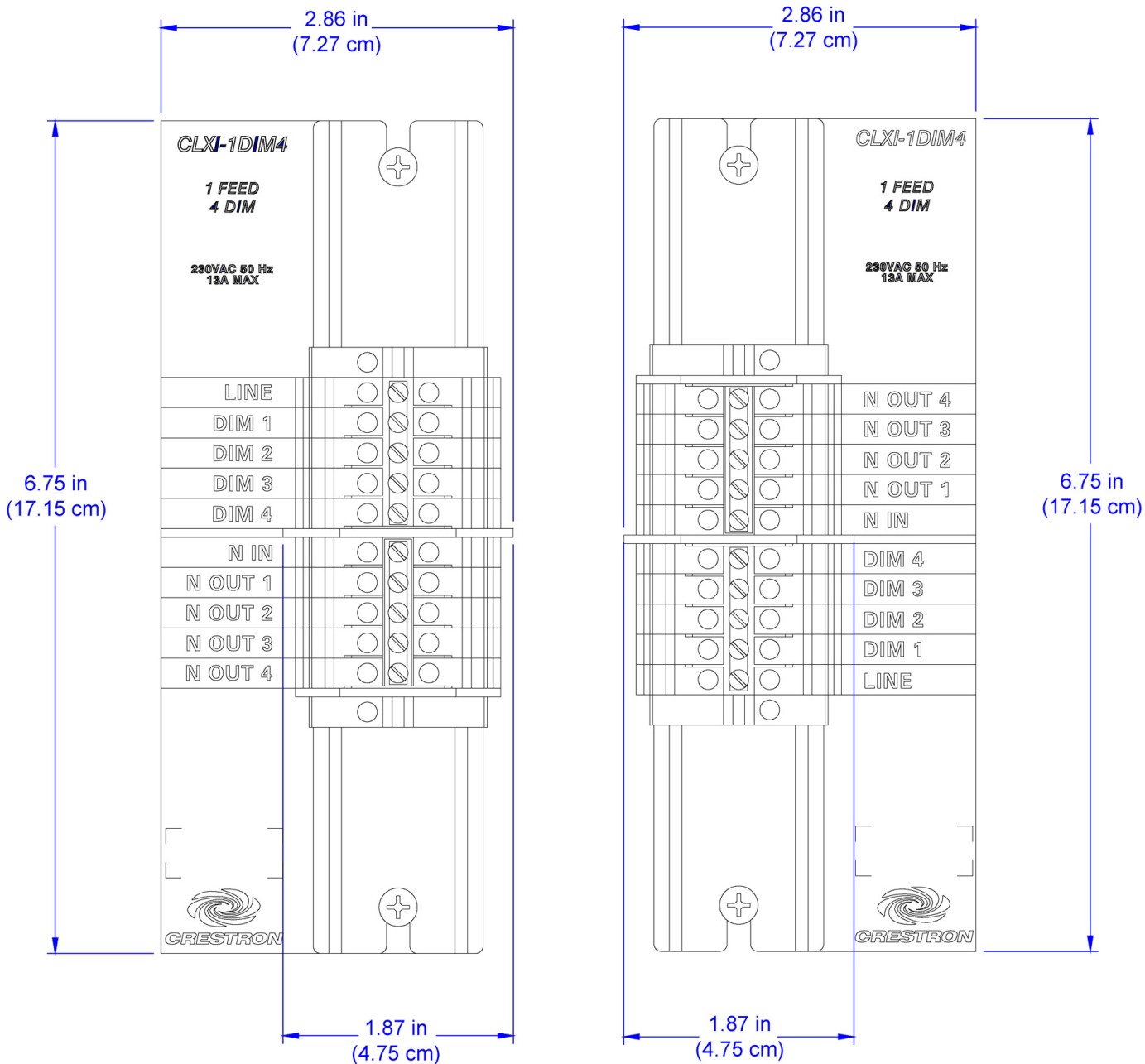
Right Side
